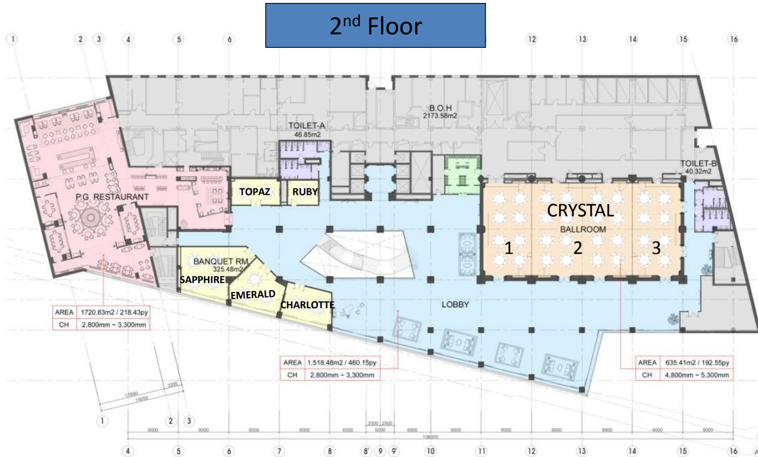
2F FLOOR PLAN
